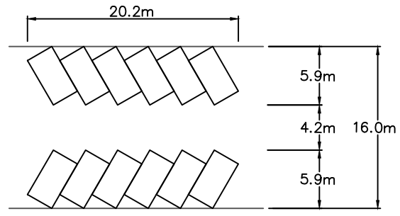
60° PARKING
