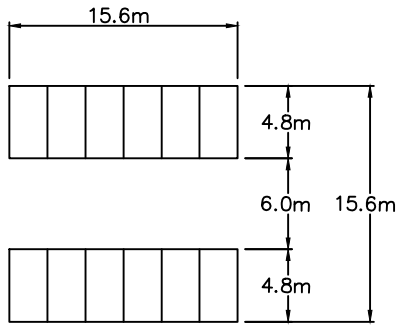
90° PARKING
