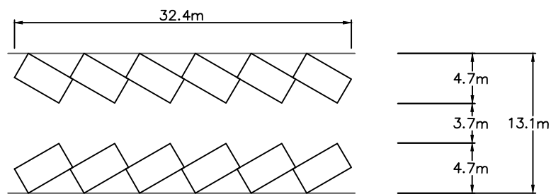
30° PARKING
