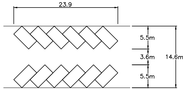
45° PARKING
